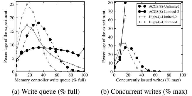
Figure 5: Write queue occupancy and write concurrency distributions.
