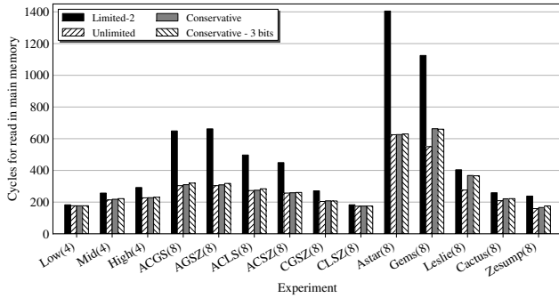
Figure 7: Read latency for read requests to main memory.
