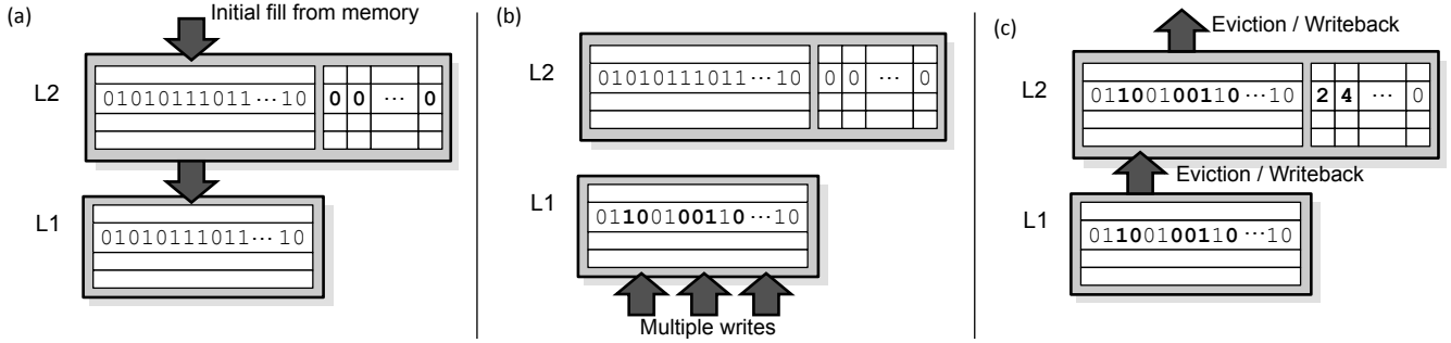
Figure 3: Token cost estimation and flow of a cache line through the memory subsystem. When the line is originally loaded from memory, (a) the counters are reset to zero. (b) The L1 cache modifies the line, but does not write it back immediately, so the values in the L1 and L2 caches differ. (c) The line is eventually written back to the L2 cache and the counters are updated based on differences in the data. When the last level cache (L2 in this case) writes back the line, it sends the memory controller the value of the accumulated counters for the line, as an estimate of the number of modified bits.
