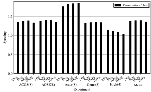
Figure 9: Sensitivity to L2 cache size.
