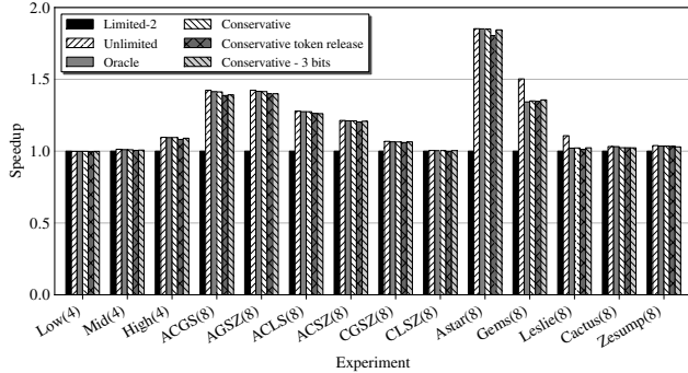
Figure 4: Speedup over limited-2 for all experiments.
