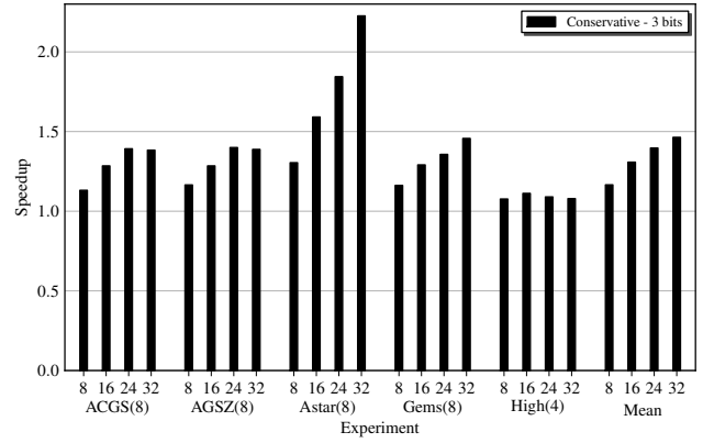
Figure 12: Sensitivity to memory controller input queue size.
