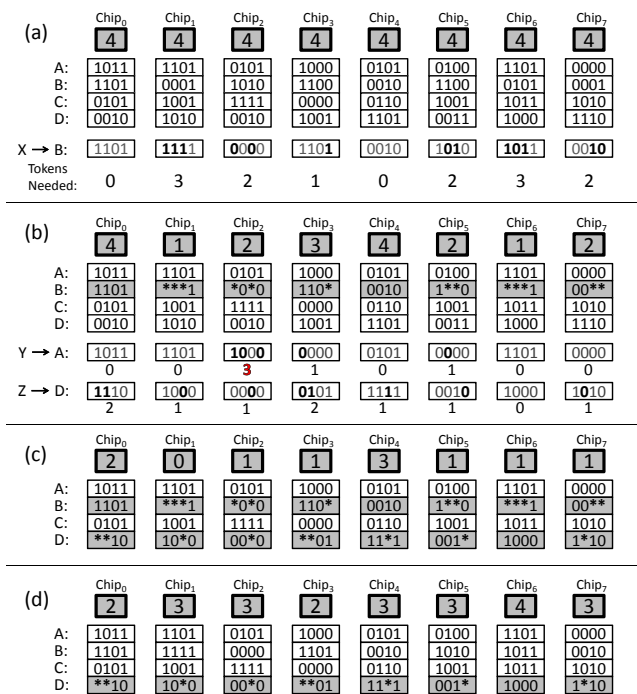
Figure 2: A token-based PCM power management example. There are logical banks (A-D) spread across the eight chips. Each chip can support at most four concurrent bit writes. Banks currently being written to are shaded, and bits actively being modified are indicated with asterisks. (a) A write operation that modifies 13 bits. (b) The write issues and decrements the token counters. There are two more writes waiting to issue, of which only one has enough tokens in all banks. (c) The second write issues and decrements the token counters. (d) The first write completes and returns the tokens it was using.
