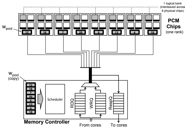
Figure 1: Block diagram of single rank of a general power-aware PCM memory architecture. The logical memory bank is composed of eight physical banks across eight separate PCM chips. As power is constrained on a per-chip basis, a pool of active counters per chip is maintained by the scheduler.
