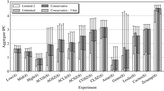
Figure 6: Aggregate IPC for all experiments.
