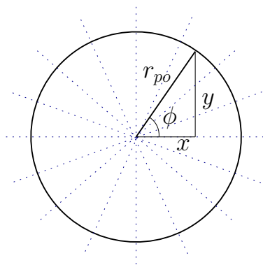
Fig. 2 Geometrical setup for finding the PRC for a general radial isochron clock. Sample isochrons are shown as dotted lines
