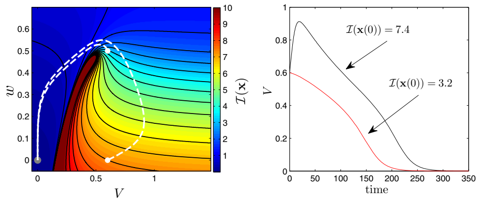
Fig. 8 The left panel shows isostable coordinates of (50) numerically calculated according to (49). Black lines denote level sets of isostables. Dashed white lines show two different trajectories starting from different initial conditions and ultimately approaching the fixed point (gray dot). In the right panel, the black trace takes longer to return to the fixed point than the red trace, as predicted from their initial isostable coordinate values
