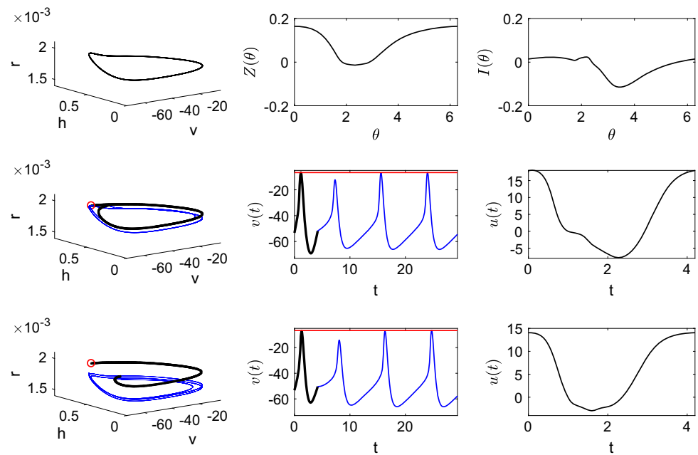
Fig. 20 Thalamic neuron model: Top row shows the uncontrolled periodic orbit, PRC, and IRC for the thalamic neuron model with parameters given in the main text. The middle (resp., bottom) row shows the trajectory, time series, and control input for control based on the augmented (resp., standard) phase reduction. Control is on (resp., off) for the portion shown by the thick black (resp., thin blue) line. The trajectory starts at the small red circle. The red horizontal line shows the amplitude of the uncontrolled periodic orbit (color figure online)
